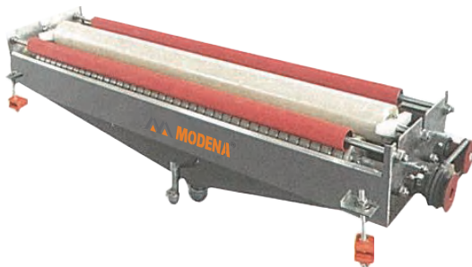
整条式底浆机 Engobing Unit (Complete Roller Type)
